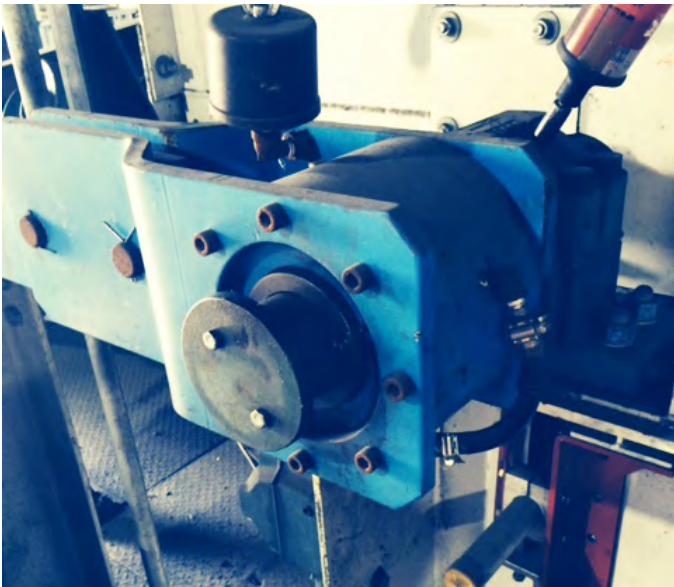
Low Speed Backstop FRHD 700
