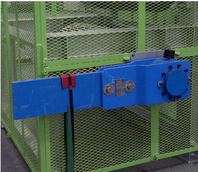
Low Speed Backstop FRHD 800
